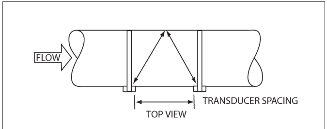
V Method Transducer Spacing
